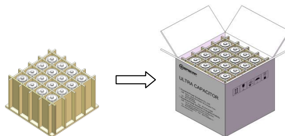
Package Drawing
